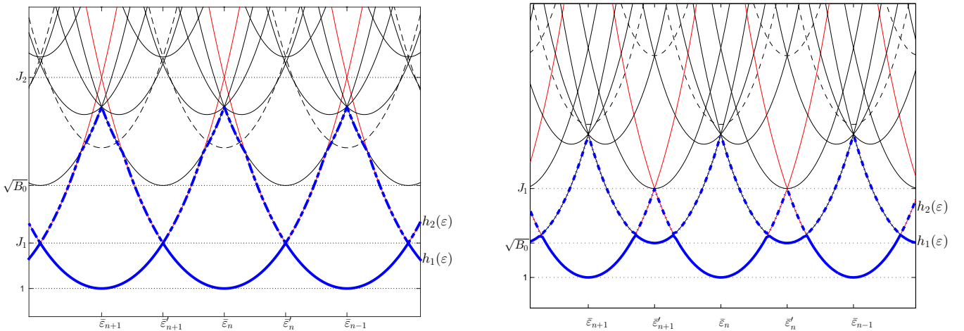
Figure 2: Graphs of the functions h_1(\varepsilon) and h_2(\varepsilon) for two metallic-colored ratios, (a) \Omega = [1, 3] (a golden-colored ratio); (b) \Omega = [2, 3] (a silver-colored ratio).
