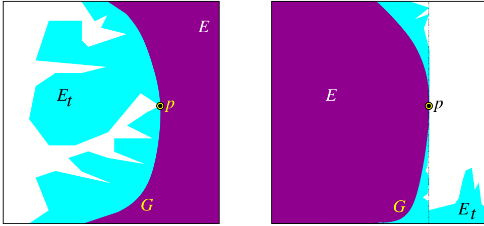
FIGURE 1. The alternative in (4.17) and (4.18).
