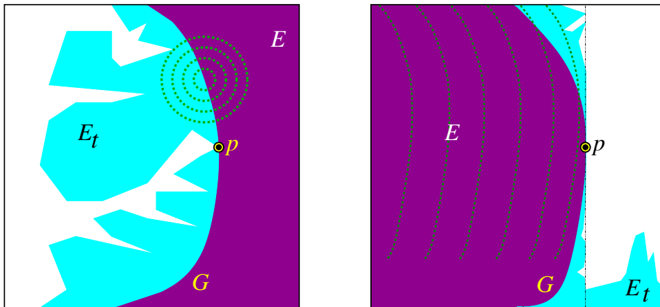
FIGURE 2. Touching \partial E_t , according to the alternative in (4.17) and (4.18).
