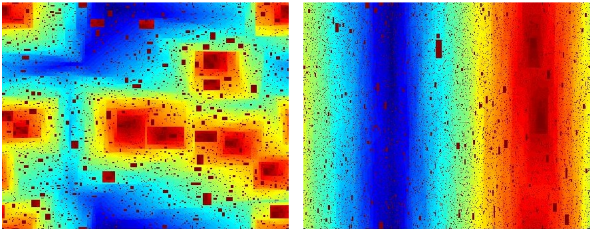
Figure 1: Left: An example of a simple bootstrap percolation's growth (red sites are the oldest, blue the youngest). Right: An example of the model's growth.
