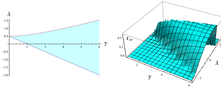
FIGURE 4. In the figure on the left, the blue area represents the domain of (\lambda, \gamma) with 1 \leq \gamma \leq 6 , where the (zero-temperature) Cooper pair condensate density r_\infty is non-zero at \mu = 1 and h = 0 . The figure on the right represents a 3D illustration of r_\infty when 1 \leq \gamma \leq 6 and -2.5 \leq \lambda \leq 2.5 with again \mu = 1 , h = 0 .
