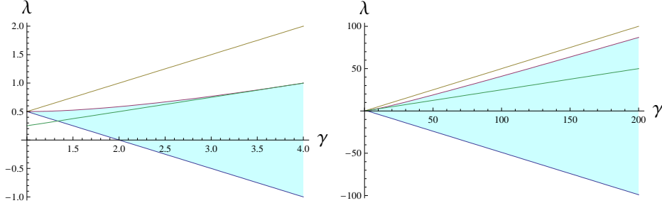
FIGURE 9. In both figures, the blue area represents the domain of (\lambda, \gamma) , where there is a superconducting phase at zero temperature for \mu = 1 and h = 0 . The two increasing straight lines (green and brown) are \gamma = 4\lambda and \gamma = 2\lambda for \gamma \geq 1 . In particular, between these two lines ( 2\lambda < \gamma < 4\lambda ), there is a superconducting–Mott–Insulator phase transition by tuning \mu .
