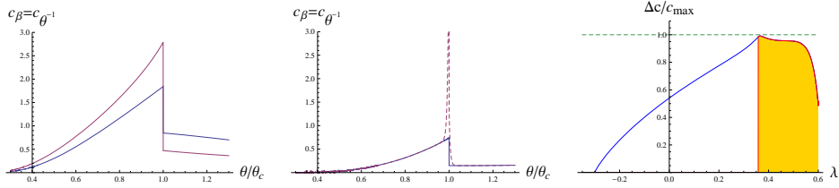
FIGURE 12. Here \mu = 1 , \gamma = 2.6 and h = 0 . Assuming \mathfrak{C}_\beta = 0 , we give 3 plots of the specific heat c_\beta as a function of the ratio \theta/\theta_c between \theta := \beta^{-1} and the critical temperature \theta_c for \lambda = 0, 0.5 (both left figure, respectively blue and red lines, second order phase transition), and \lambda = 0.575 (figure on the center, blue line, first order phase transition). The dashed red line in the figure on the center indicates what the specific heat at finite volume might be since c_{\theta_c^{-1}} = +\infty . The right figure is a plot as a function of \lambda of the relative specific heat jump, i.e., the ratio \Delta c/c_{\max} between the jump \Delta c at \theta = \theta_c and the maximum value c_{\max} of c_{\theta_c^{-1}} at the same point. The yellow colored area indicates that this ratio numerically computed is formally infinite due to a first order phase transition.
