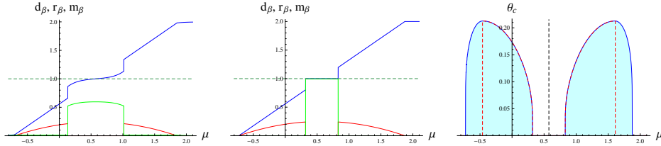
FIGURE 10. Here \lambda = 0.575 , \gamma = 2.6 , and h = 0.1 . In the two figures on the left, we plot the electron density d_\beta (blue line), the Cooper pair condensate density r_\beta (red line) and the magnetization density m_\beta (green line) as functions of \mu for \beta = 7 (left figure) or 30 (low temperature regime, figure on the center). Observe the superconducting–Mott Insulator phase transition which appears in both cases. In the right figure, we illustrate as a function of \mu the corresponding critical temperature \theta_c . The blue line corresponds to a second order phase transition, whereas the red dashed line represents the domain of \mu with first order phase transition. The black dashed line is the chemical potential \mu = \lambda corresponding to an electron density per site equal to 1.
