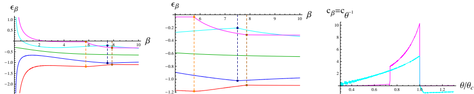
FIGURE 16. In the two figures on the left, we give illustrations of the mean energy per site \epsilon_\beta as a function of the inverse temperature \beta for densities \rho = 0.7 (magenta line), 0.9 (cyan line), 1 (green line), 1.1 (blue line) and 1.3 (red line). For \rho = 1 , there is no phase transition and for \rho = 0.9 or 1.1 only a ferromagnetic–superconducting phase appears, whereas for \rho = 0.7 or 1.3 this last phase is followed for larger \beta by a superconducting phase. In the figure on the right, assuming \mathfrak{C}_\beta = 0 , we give two plots of the specific heat c_\beta as a function of the ratio \theta/\theta_c between \theta := \beta^{-1} and the critical temperature \theta_c for densities \rho = 0.7 (magenta line) and 0.9 (cyan line). In all figures, \lambda = 0.575 , \gamma = 2.6 , and h = 0.1 .
