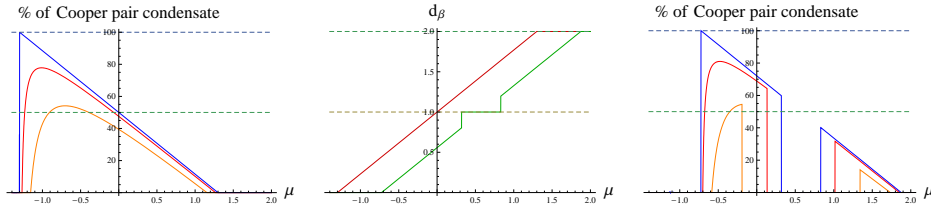
FIGURE 8. The fraction of electron pairs in the condensate is given in right and left figures as a function of \mu . In the figure on the left, \lambda = h = 0 , with inverse temperatures \beta = 2.45 (orange line), 3.45 (red line) and 30 (blue line). In the figure on the right, \lambda = 0.575 and h = 0.1 with \beta = 5 (orange line), 7 (red line) and 30 (blue line). The figure on the center illustrates the electron density d_\beta also as a function of \mu at \beta = 30 (low temperature regime) for \lambda = h = 0 (red line) and for \lambda = 0.575 and h = 0.1 (green line). In all figures, \gamma = 2.6 .
