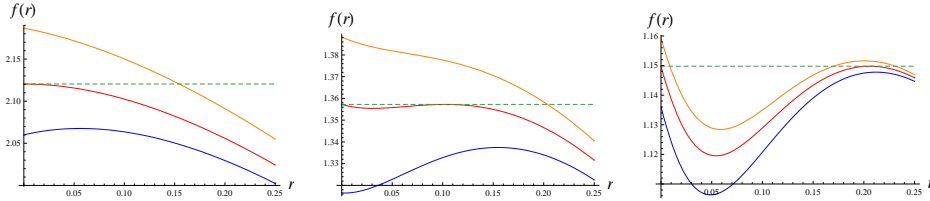
FIGURE 18. Illustrations of the function f(r) for r \in [0, 1/4] at (\mu, \gamma, h) = (1, 2.6, 0) with inverse temperatures \beta = \beta_c - 0.3 (orange line), \beta = \beta_c (red line), \beta = \beta_c + 0.5 (blue line), and with coupling constants \lambda = 0 (left figure), \lambda = 0.45 (figure on the center) and \lambda = 0.575 (right figure). Here \beta_c = \theta_c^{-1} is the critical inverse temperature which, from left to right, equals 2.04, 3.46 and 6.35 respectively.
