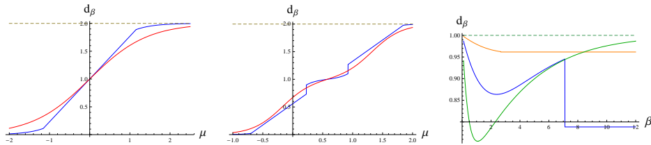
FIGURE 5. In the figures on the left, we give illustrations of the electron density d_\beta as a function of the chemical potential \mu for \beta < \beta_c (red line) and \beta > \beta_c (blue line) at coupling constant \lambda = 0 (figure on the left, \beta = 1.4, 2.45 ) and \lambda = 0.575 (figure on the center, \beta = 4, 6.45 ). In the figure on the right, d_\beta is given as a function of \beta at \mu = 0.3 with \lambda > \mu equal to 0.35 (orange line, second order phase transition), 0.575 (blue line, first order phase transition) and 1.575 (green line, no phase transition). In all figures, \gamma = 2.6 , h = 0 and \beta_c = \theta_c^{-1} is the critical inverse temperature.
