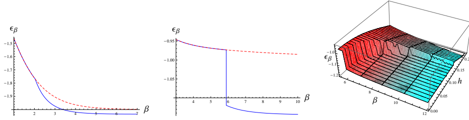
FIGURE 11. In the two figures on the left, we give the mean energy per site \epsilon_\beta as a function of \beta at h = 0 for \lambda = 0 (figure on the left, second order BCS phase transition) or \lambda = 0.575 (figure on the center, first order phase transition). The dashed line in both figures is the mean energy per site with zero Cooper pair condensate density. On the right figure, \epsilon_\beta is given as a function of \beta and h at \lambda = 0.575 . The color from red to blue reflects the decrease of the temperature and the plateau corresponds to the superconducting phase. In all figures, \mu = 1 and \gamma = 2.6 .
