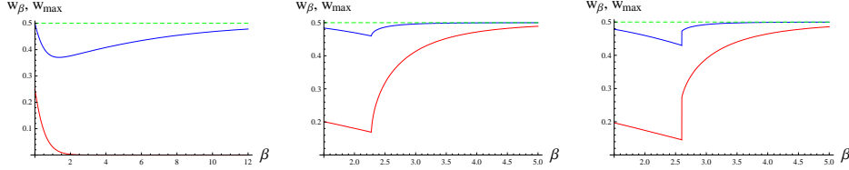
FIGURE 7. Illustration of the Coulomb correlation density w_\beta (red lines) and its corresponding upper bound w_{\max} (blue lines) as a function of \beta > 0 at \mu = 0.2 , \gamma = 2.6 , for \lambda = 1.305 < \mu (left figure, d_\beta < 1 ), \lambda = 0.2 = \mu (two right figures, d_\beta = 1 ), and from the left to the right, with h = 0 ( m_\beta = 0 ), and h = 0.3, 0.35 (where m_\beta > 0 ). The dashed green lines indicate that d_\infty/2 = 0.5 in the three cases. In the figure on the left there is no superconducting phase in opposition to the right figures where we see a phase transition for \beta > 2.3 (second order) or 2.6 (first order).
