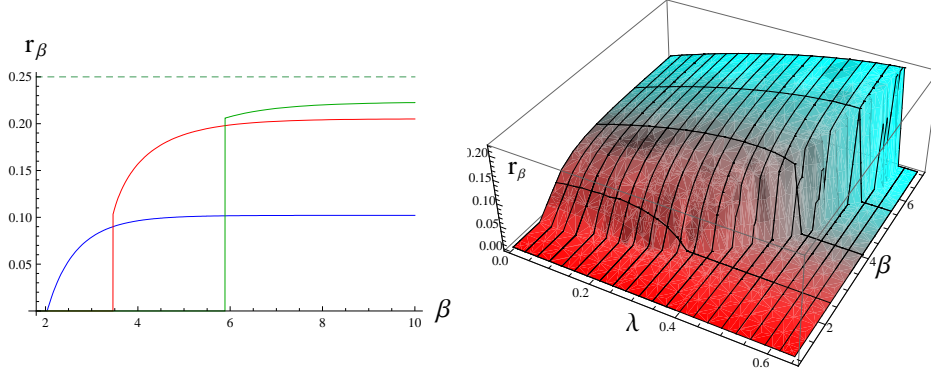
FIGURE 3. In the figure on the left, we have three illustrations of the Cooper pair condensate density r_\beta as a function of the inverse temperature \beta for \lambda = 0 (blue line), \lambda = 0.45 (red line) and \lambda = 0.575 (green line). The figure on the right represents a 3D illustration of r_\beta as a function of \lambda and \beta . The color from red to blue reflects the decrease of the temperature. In all figures, \mu = 1 , \gamma = 2.6 and h = 0 .
