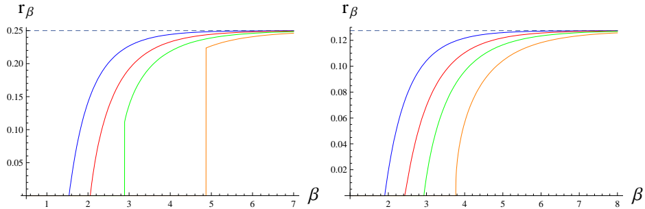
FIGURE 13. Illustrations of the Cooper pair condensate density r_\beta as a function of the inverse temperature \beta for \gamma = 2.6 , h = 0 , and densities \rho = 1, 1.7 (respectively left and right figures), with \lambda = 0 (blue line), 0.5 (red line), 0.75 (green line), and 1 (orange line). The dashed line indicates the value of r_\infty .
