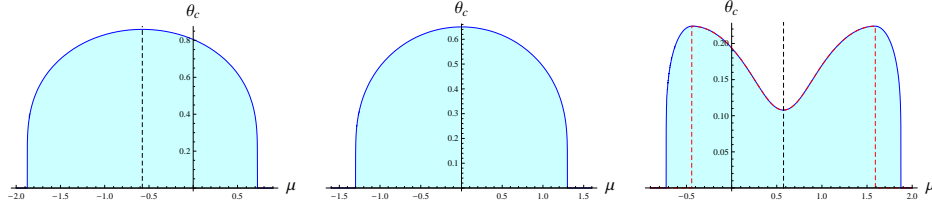
FIGURE 1. Illustration, as a function of \mu , of the critical temperature \theta_c = \theta_c(\mu, \lambda, \gamma, h) such that r_\beta > 0 if and only if \beta > \theta_c^{-1} (blue area) for \gamma = 2.6 , h = 0 and with \lambda = -0.575 (left figure), 0 (figure on the center) and 0.575 (right figure). The blue line corresponds to a second order phase transition, whereas the red dashed line represents the domain of \mu with a first order phase transition. The black dashed line is the chemical potential \mu = \lambda corresponding to an electron density per site equal to 1, see Section 3.
