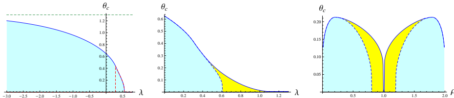
FIGURE 15. Illustration, as a function of \lambda (the two figures on the left) or \rho (figure on the right), of the critical temperature \theta_c = \theta_c(\rho, \lambda, \gamma, h) for \gamma = 2.6 , h = 0.1 and with \rho = 1 (left figure), \rho = 0.7 (figure on the center) and \lambda = 0.575 (right figure). The blue and yellow area correspond respectively to the superconducting and ferromagnetic–superconducting phases, whereas the red dashed line indicates the domain of \lambda with a first order phase transition as a function of \beta or the temperature \theta := \beta^{-1} (It only exists in the left figure). The dashed green line (left figure) is the asymptote when \lambda \rightarrow -\infty . In the right figure, observe that there is no phase transition for \rho = 1 .
