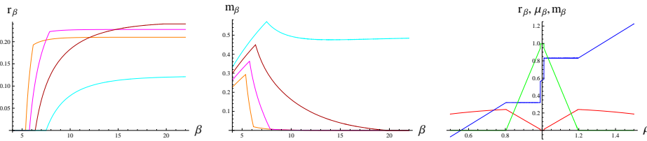
FIGURE 14. In the two figures on the left, we give illustrations of the Cooper pair condensate density r_\beta and the magnetization density m_\beta as functions of the inverse temperature \beta for densities \rho = 0.6 (orange line), 0.7 (magenta line), 0.8 (red line), 0.9 (cyan line). In the figure on the right, we illustrate the coexistence of ferromagnetic and superconducting phases via graphs of r_\beta , m_\beta and the chemical potential \mu_\beta as functions of \rho for \beta = 30 (low temperature regime). In all figures, \lambda = 0.575 , \gamma = 2.6 , and h = 0.1 . (The small discontinuities around \rho = 1 in the right figure are numerical anomalies)
