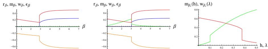
FIGURE 17. In the two figures on the left, we give illustrations of the Cooper pair condensate density r_\beta (blue line), the magnetization density m_\beta (green line), the Coulomb correlation density w_\beta (red line), and the mean–energy per site \epsilon_\beta (orange line) as functions of the inverse temperature \beta for h = 0 (figure on the left) and h = 0.1 (figure on the center) whereas \mu_\beta = \lambda = 0.375 , i.e., \rho = 1 . In the figure on the right, we illustrate m_{\beta_c} (green line) and w_{\beta_c} (red line) respectively as functions of h with \mu = \lambda = 0.375 and \lambda with (\mu, h) = (0.375, 0.1) at the critical inverse temperature \beta_c := \theta_c^{-1} \simeq 3.04 .
