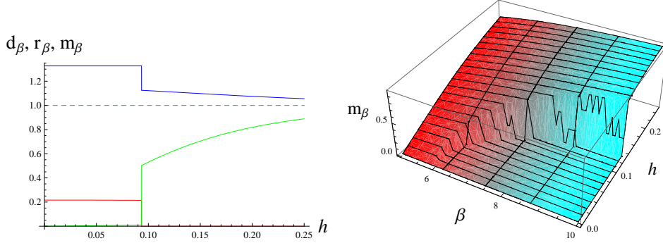
FIGURE 6. In the figure on the left, we have an illustration of the electron density d_\beta (blue line), the Cooper pair condensate density r_\beta (red line) and the magnetization density m_\beta (green line) as functions of the magnetic field h at \beta = 7 , \mu = 1 , \lambda = 0.575 and \gamma = 2.6 . The figure on the right represents a 3D illustration of m_\beta = m_\beta(1, 0.575, 2.6, h) as a function of h and \beta . The color from red to blue reflects the decrease of the temperature. In both figures, we can see the Meißner effect (In the 3D illustration, the area with no magnetization corresponds to r_\beta > 0 ).
