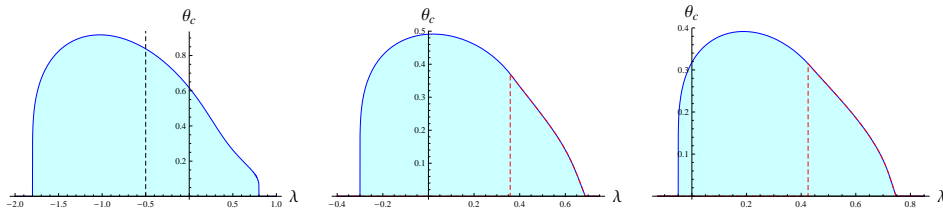
FIGURE 2. Illustration, as a function of \lambda , of the critical temperature \theta_c = \theta_c(\mu, \lambda, \gamma, h) for \gamma = 2.6 , h = 0 and with \mu = -0.5 (left figure), \mu = 1 (figure at the center) and \mu = 1.25 (right figure). The blue line corresponds to a second order phase transition, whereas the red dashed line represents the domain of \lambda with first order phase transition. The black dashed line is the coupling constant \lambda = \mu corresponding to an electron density per site equal to 1, see Section 3.
