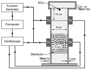
FIG. 1. A schematic diagram of the experimental apparatus is shown. Solid (dashed) lines denote the transmitted (received) electrical signal paths. The glass beads are not drawn to scale.
