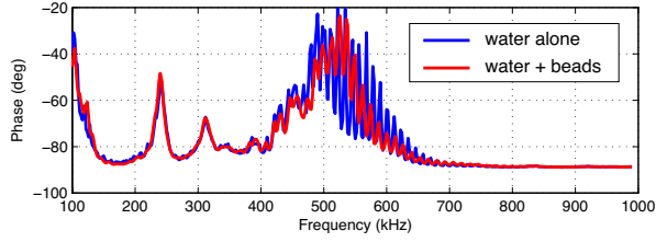
FIG. 2. (Color online) The phase of the measured electrical input impedance of one of the receiving transducers depicted in Fig. 1 is shown. The blue curve is for the transducer mounted in the apparatus when filled with water, and the red curve is for water-saturated beads. The phase difference apparent within the experimental frequency range (300 kHz through 800 kHz) was found to lead to correctable systematic errors in the sound speed measurement.
