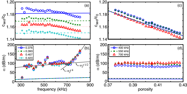
FIG. 4. (Color online) Measured sound speed ratios and attenuation coefficients of water-saturated glass beads are shown as a function of frequency in (a) and (b) and as a function of porosity in (c) and (d). Heavy dashed and solid lines correspond to the predictions of the EDFM 13 and symbols correspond to measurements. Trendlines are shown with light solid black lines in (b) to illustrate f^{1/2} dependence below 700 kHz and f^4 dependence above.
