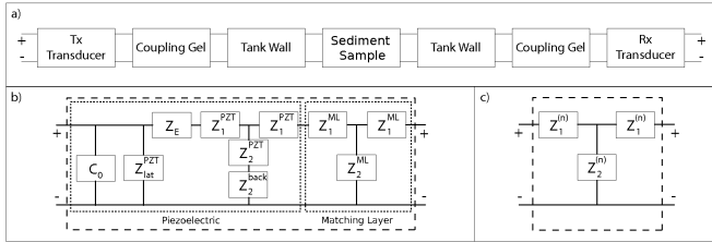
FIG. 3. A schematic of the transmission line model is shown in (a). It is composed of a Mason model for the transducers (b) and generic transmission line elements (c) for the remaining layers.
