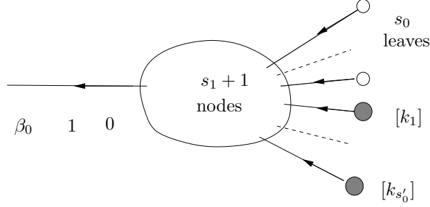
Figure 5: A tree contributing to \beta_0^{[k]} .
