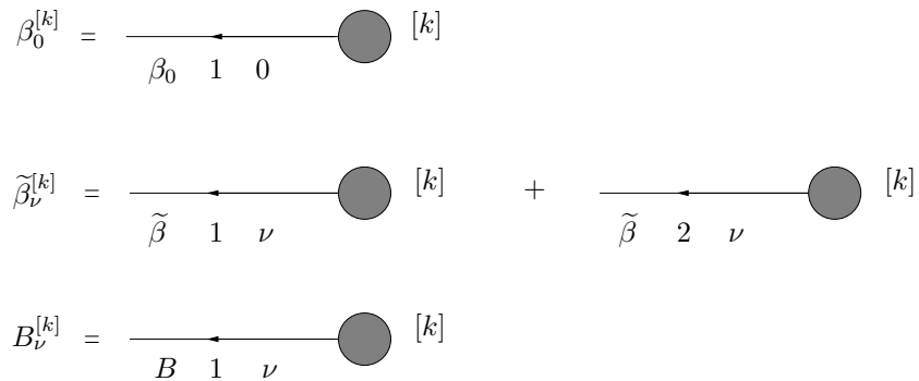
Figure 4: Graph elements.
