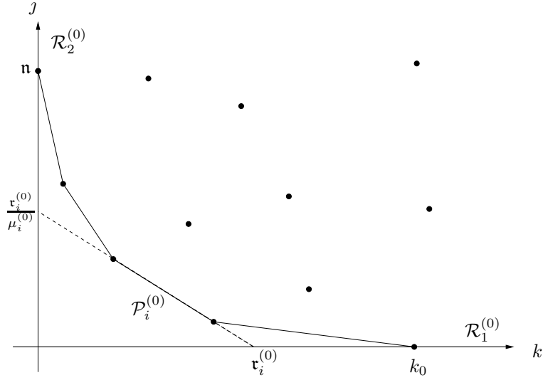
Figure 1: Newton polygon.
