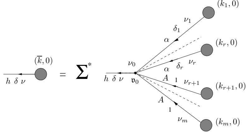
Figure 3: Graphical representation for the recursive equations (2.23).
