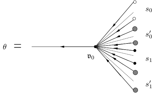
Figure 6: An allowed tree contributing to f_{h,\nu}^{[k]} .
