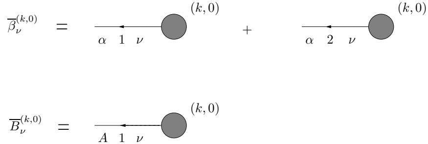
Figure 2: Graph elements.
