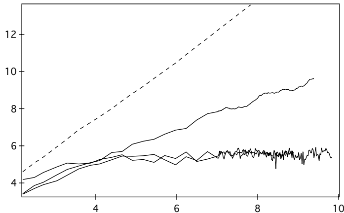
Figure 3: The moment as function of time (log – log scale) for the combination of PF with periodic sequences. The periods were 4 (dashed), 16 (line), 7 and 10 (localization).
