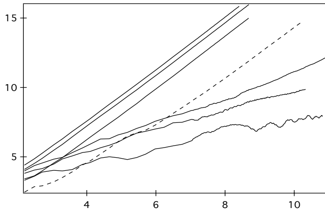
Figure 2: The moment as function of time (log – log scale) for the combination of TM with itself shifted. The dashed line is for the original TM (no shift at all).
