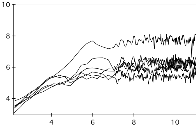
Figure 1: The moment as function of time (log – log scale) for the combination of TM and FCC substitution sequences. The sequence FCC was kept fixed, while TM was shifted by 0, 1, \dots, 5 in order to explore different elements of the product of their hulls.
