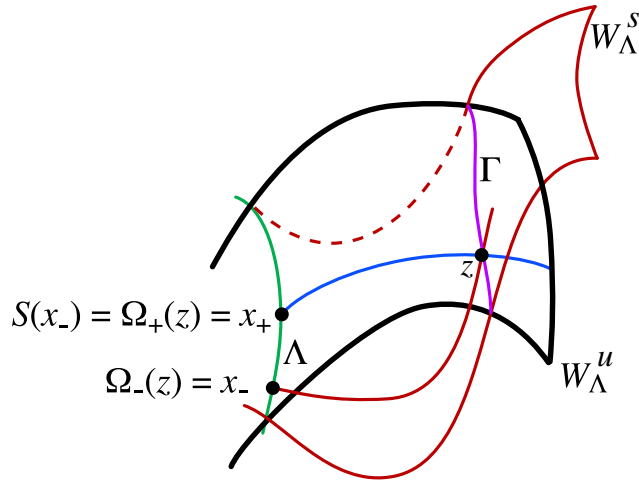
FIGURE 3. Illustration of the definition of the scattering map. Definition 5
