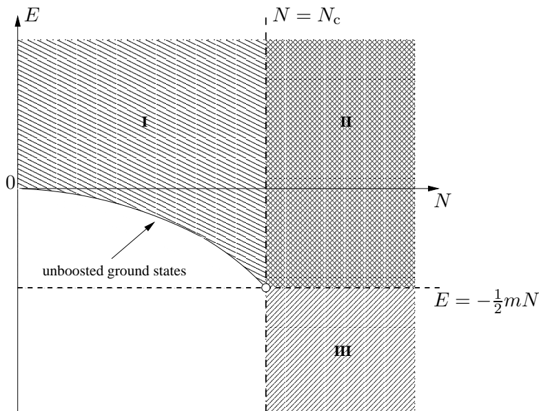
Figure 1: Qualitative diagram for the boson star equation (1.1) with positive mass parameter m > 0 . Here N = \mathcal{N}(\psi_0) and E = \mathcal{E}(\psi_0) denote charge and energy for the initial condition \psi_0 \in \mathbf{H}^{1/2}(\mathbb{R}^3) . In region I , all solutions are global in time and the (unboosted) ground states are minimizers of \mathcal{E}(\psi) subject to fixed \mathcal{N}(\psi_0) = N with 0 < N < N_c . If N exceeds N_c , the energy E can attain values below -\frac{1}{2}mN . As shown in [5] for spherically symmetric \psi_0 \in C_c^\infty(\mathbb{R}^3) that belong to region III , we have in fact blow-up of \psi(t) within a finite time. Finally, the qualitative behavior of solutions with initial conditions in region II appear to be of indefinite nature.
