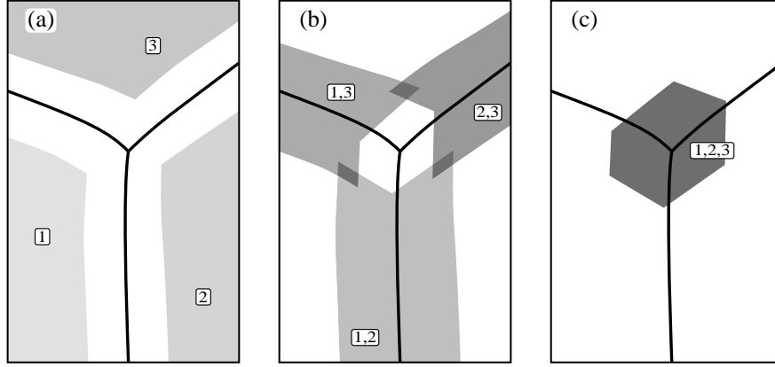
FIGURE 2. An illustration of the sets \mathcal{U}_\epsilon(Q) in the vicinity of a multiple point. The thick lines indicate the visible portion of the set of coexistence points \mathcal{G} . Three phases, here labeled 1, 2 and 3, are stable at the multiple point. In (a), the three shaded domains represent the sets \mathcal{U}_\epsilon(\{1\}) , \mathcal{U}_\epsilon(\{2\}) and \mathcal{U}_\epsilon(\{3\}) , with the label indicated by the number in the box. Similarly, in (b) the three regions represent the sets \mathcal{U}_\epsilon(\{1, 2\}) , \mathcal{U}_\epsilon(\{2, 3\}) and \mathcal{U}_\epsilon(\{1, 3\}) . Finally, (c) contains only one shaded region, representing the set \mathcal{U}_\epsilon(\{1, 2, 3\}) . The various regions \mathcal{U}_\epsilon(Q) generously overlap so that their union covers the entire box.
