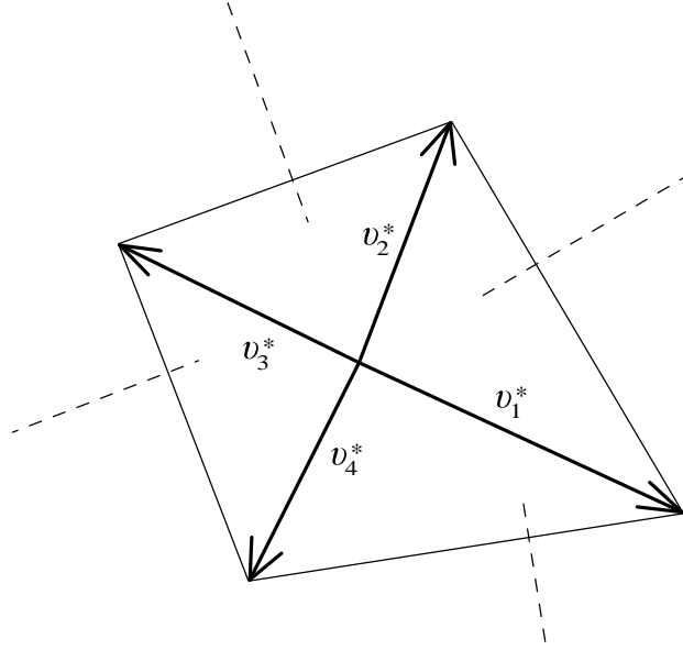
FIGURE 3. An illustration of the situation around a quadruple point. Here v_1^*, \dots, v_4^* are the complex conjugates of the quantities from (2.4) and q_1 = q_2 = q_3 < q_4 . (The quadruple point lies at the common tail point of the vectors v_1^*, \dots, v_4^* .) The dashed lines indicate the asymptotes of the “strings” of zeros sufficiently far—on the scale L^{-d} —from the quadruple point. Note the lateral shift of these lines due to the fact that q_4 > q_1, q_3 . The picture seems to suggest that, on the scale L^{-d} , the quadruple point splits into two triple points.
