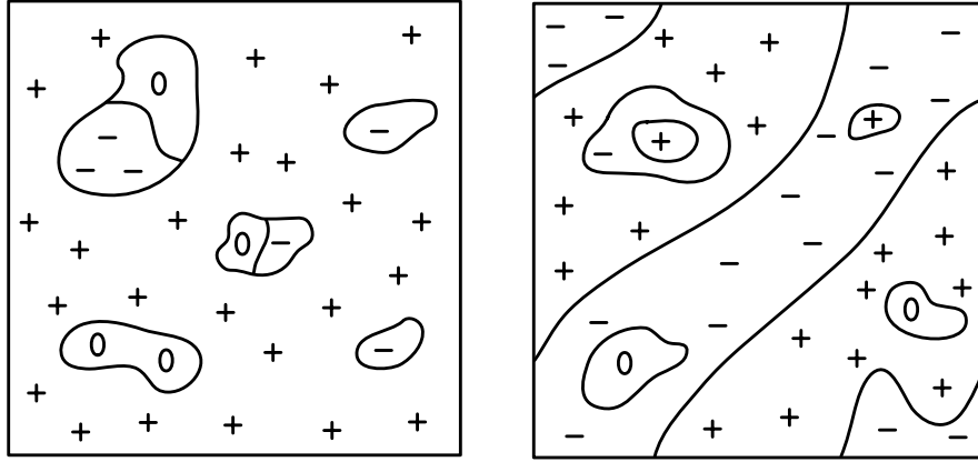
FIGURE 1. Schematic examples of configurations, along with their associated contours, which contribute to different terms in the decomposition in (1.6). Here we have a spin model with r = 3 equilibrium phases denoted by + , - and 0 . The configuration on the left has all contours smaller than the cutoff—which we set to L/3 where L is the side of the box—and will thus contribute to Z_+^{(L)} because + is the external phase for all external contours. The configuration on the right has long contours and will be assigned to the error term.
